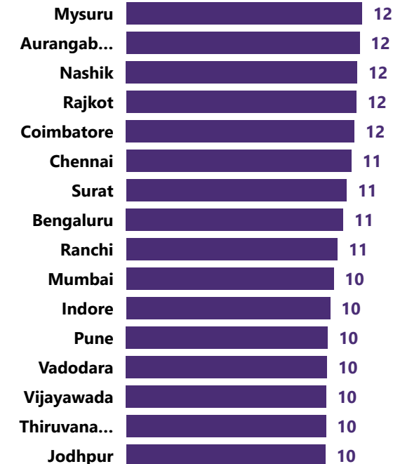
Avg_Wind_Speed_kmh by City
