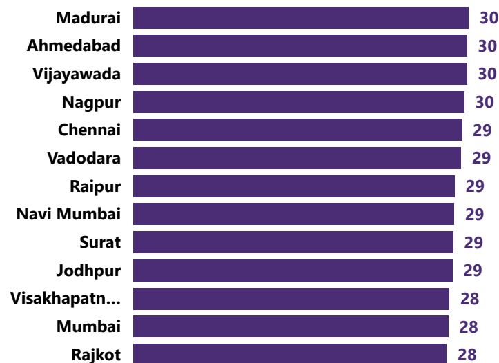
Avg_Temp_C by City
