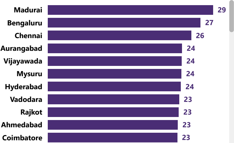
Avg_Visibility_km by City
